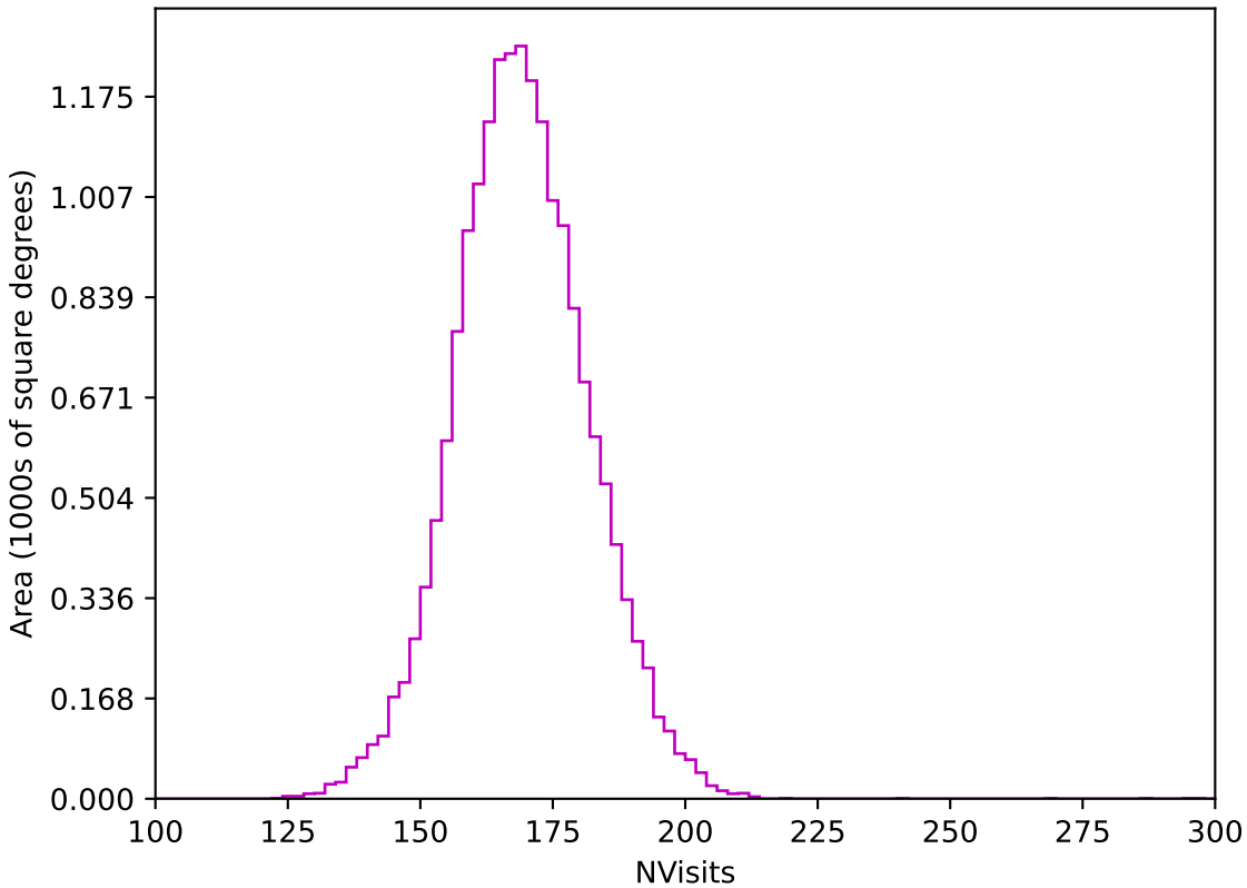
noroll_mjdp60_v3.4_10yrs WFD z band: NVisits
