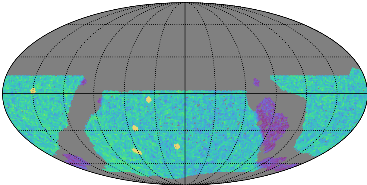
noroll_mjdp60_v3.4_10yrs WFD u band: NVisits
