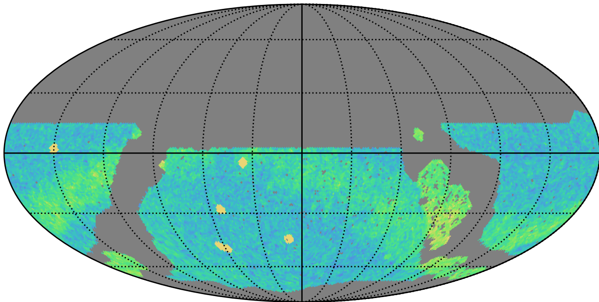
noroll_mjdp60_v3.4_10yrs WFD r band: NVisits
