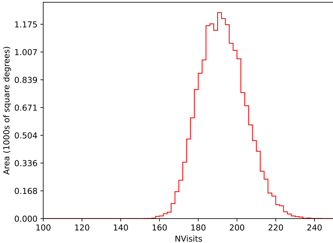
noroll_mjdp60_v3.4_10yrs WFD i band: NVisits
