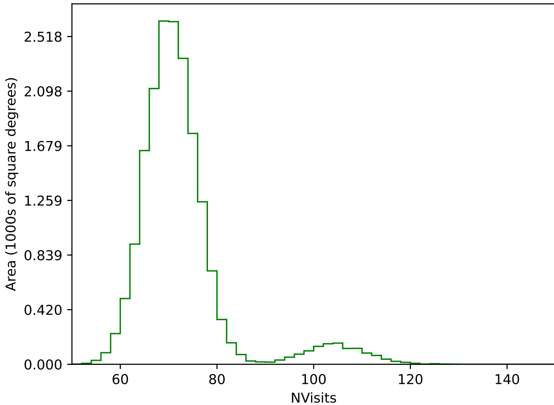
noroll_mjdp60_v3.4_10yrs WFD g band: NVisits
