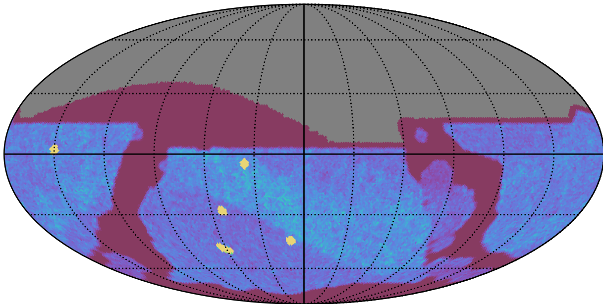
noroll_mjdp60_v3.4_10yrs All sky z band: NVisits
