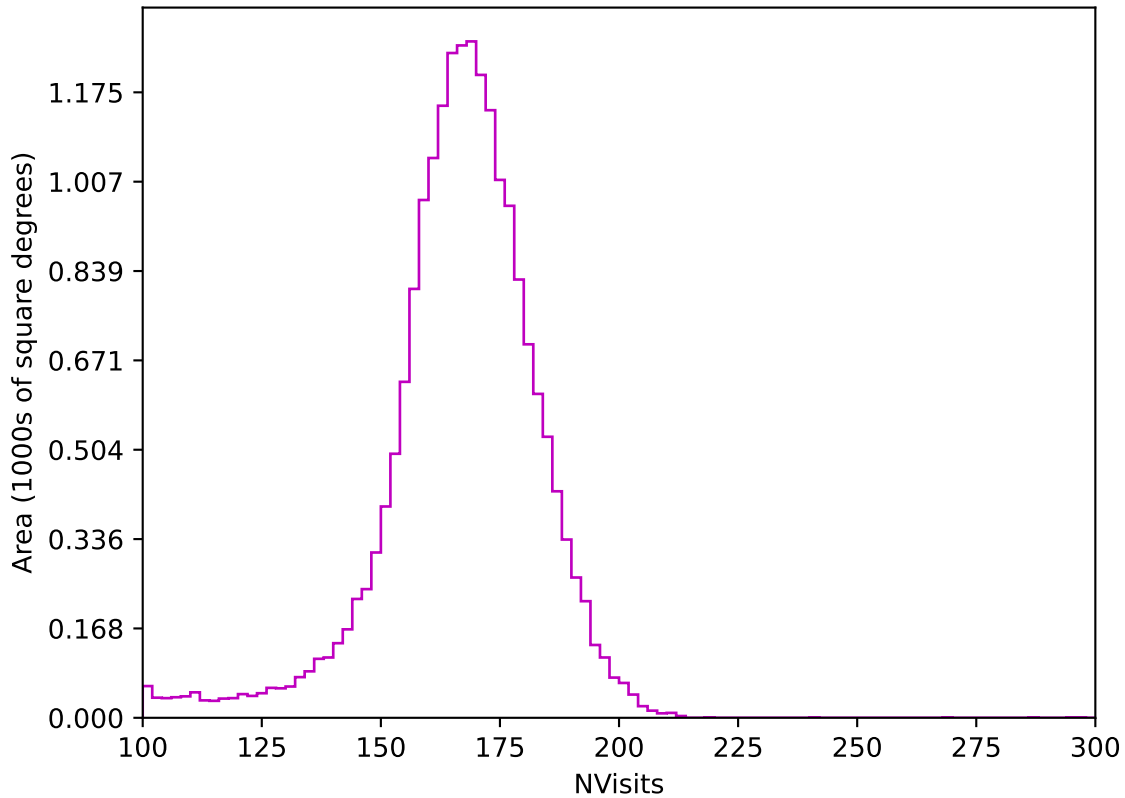
noroll_mjdp60_v3.4_10yrs All sky z band: NVisits
