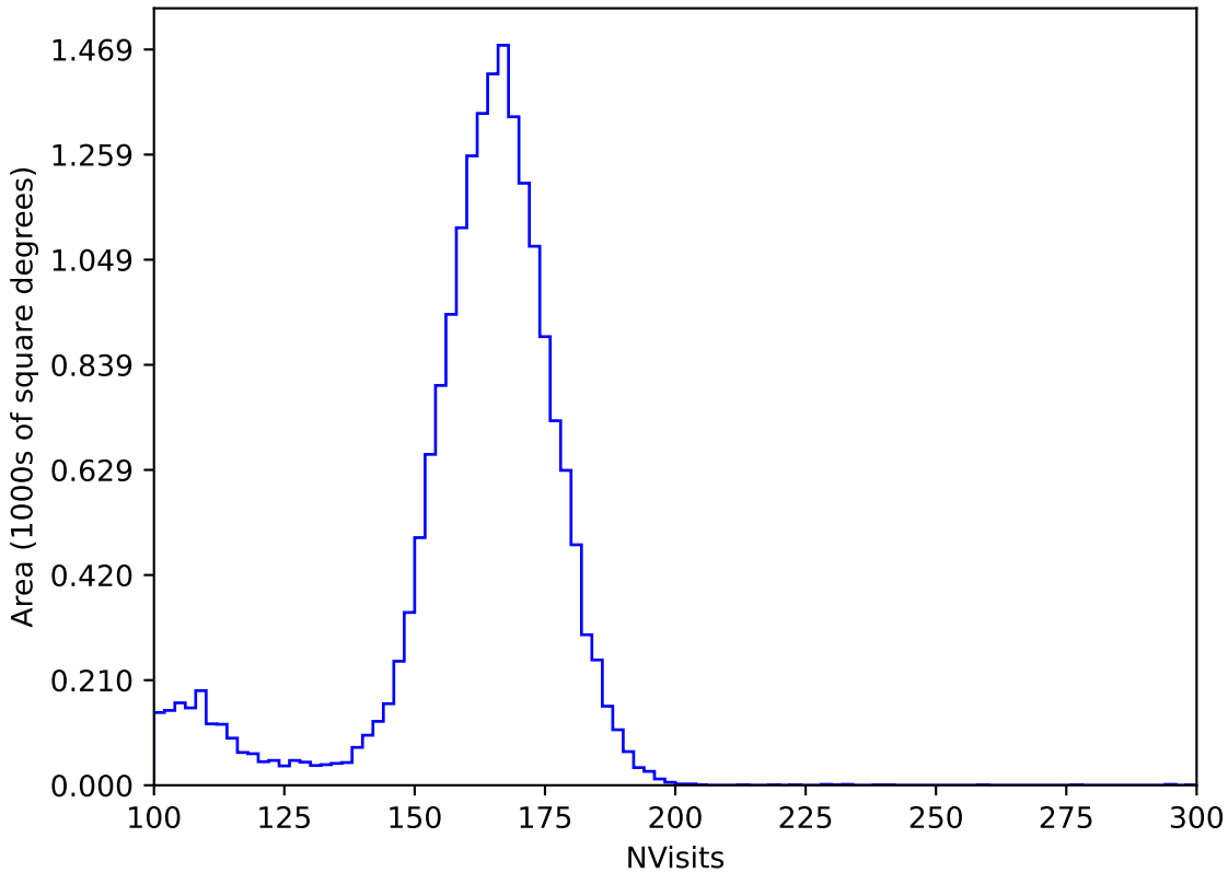
noroll_mjdp60_v3.4_10yrs All sky y band: NVisits
