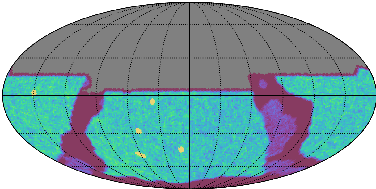
noroll_mjdp60_v3.4_10yrs All sky u band: NVisits
