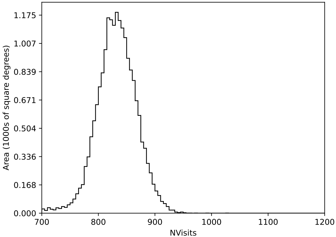
noroll_mjdp60_v3.4_10yrs All sky all bands: NVisits
