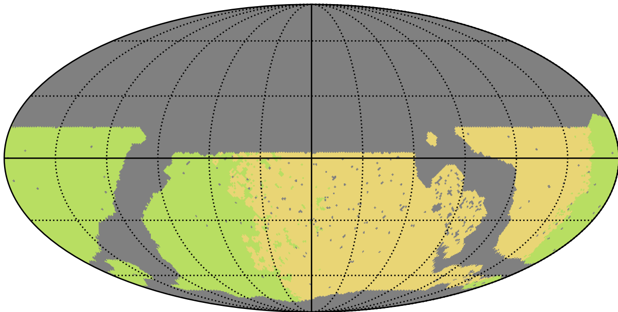
noroll_mjdp60_v3.4_10yrs WFD all bands: NSeasons
