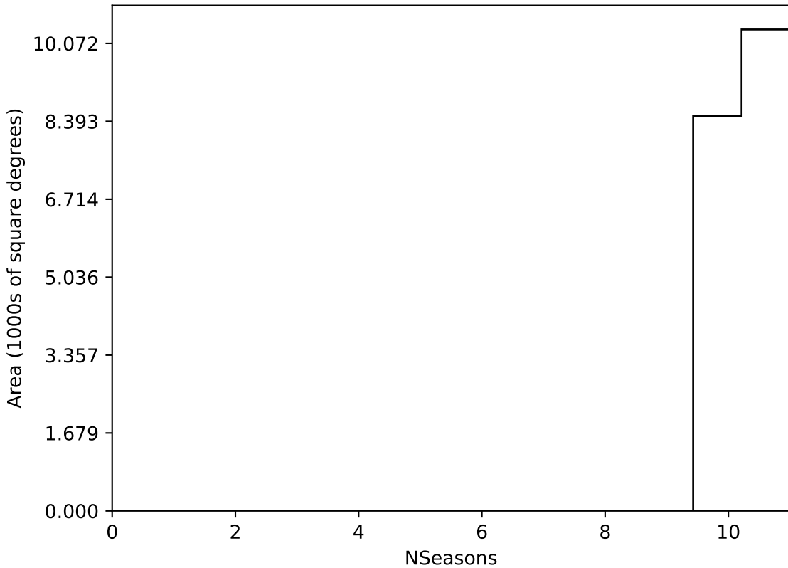
noroll_mjdp60_v3.4_10yrs WFD all bands: NSeasons
