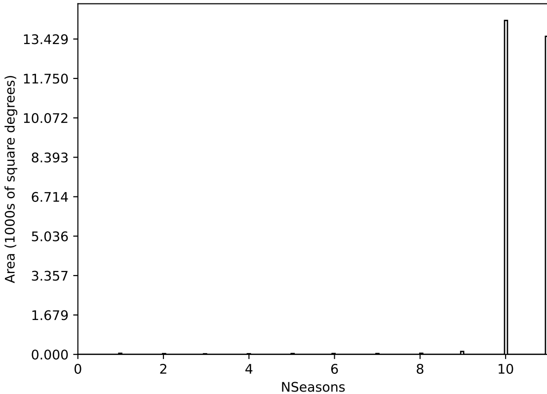
noroll_mjdp60_v3.4_10yrs All sky all bands: NSeasons
