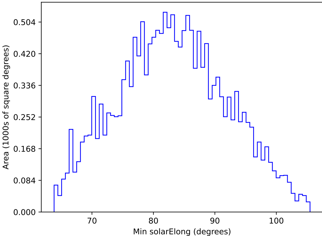
noroll_mjdp60_v3.4_10yrs WFD u band: Min solarElong
