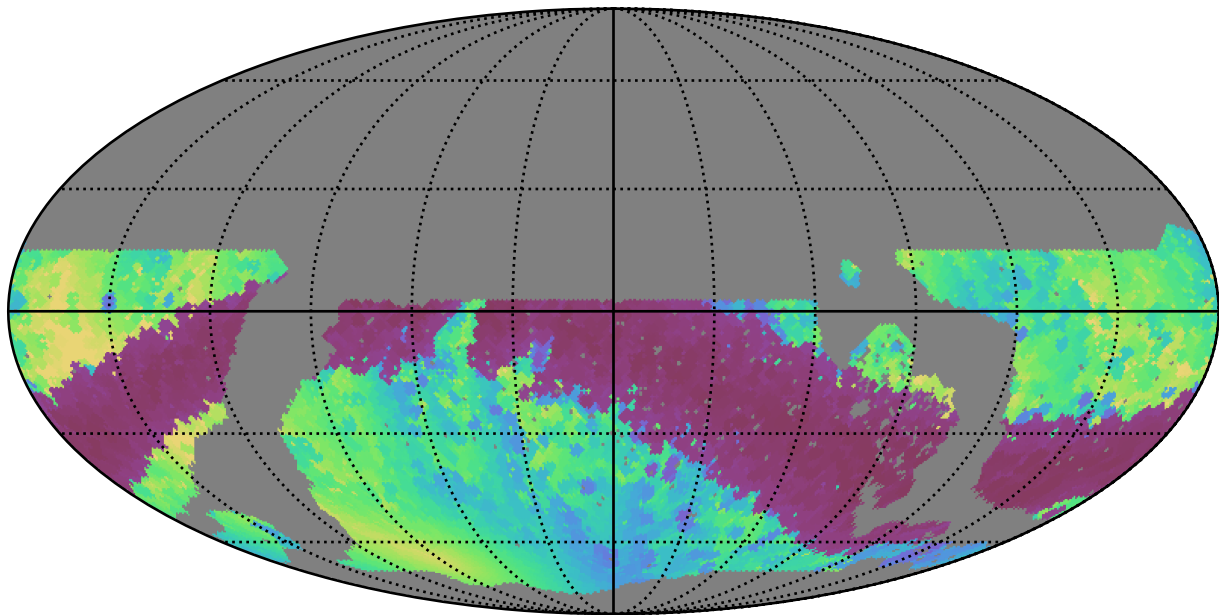
noroll_mjdp60_v3.4_10yrs WFD r band: Min solarElong
