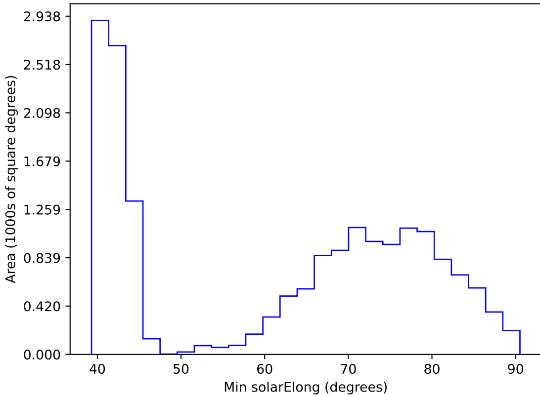
noroll_mjdp60_v3.4_10yrs WFD r band: Min solarElong
