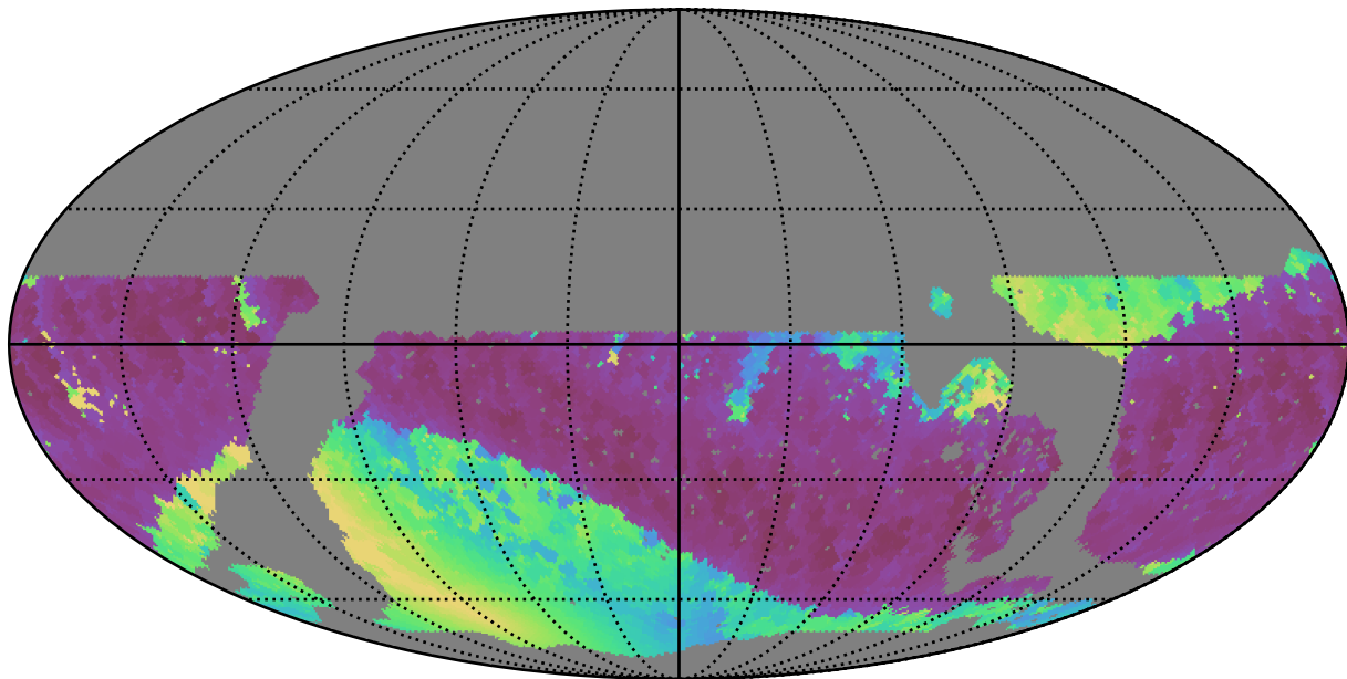
noroll_mjdp60_v3.4_10yrs WFD i band: Min solarElong
