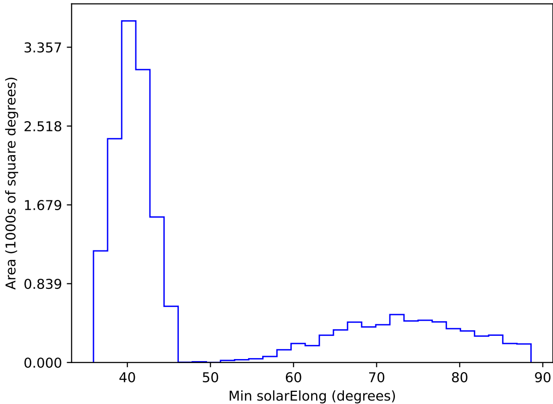
noroll_mjdp60_v3.4_10yrs WFD i band: Min solarElong
