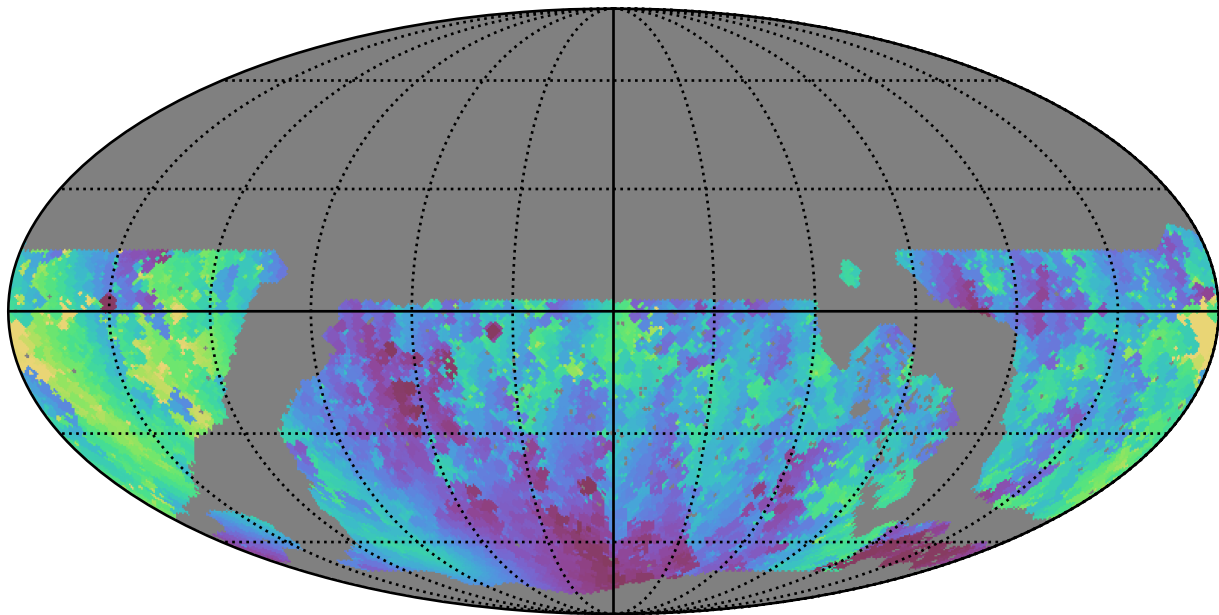
noroll_mjdp60_v3.4_10yrs WFD g band: Min solarElong
