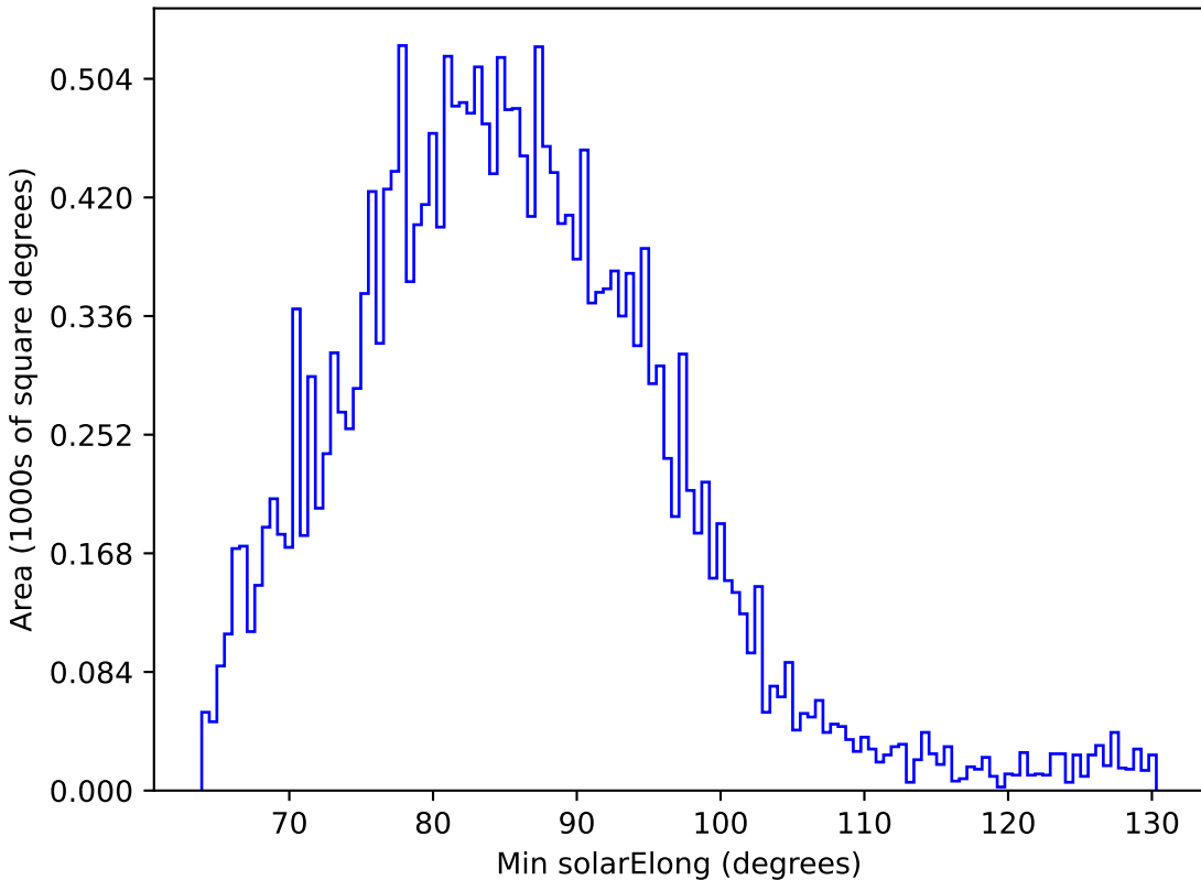
noroll_mjdp60_v3.4_10yrs All sky u band: Min solarElong
