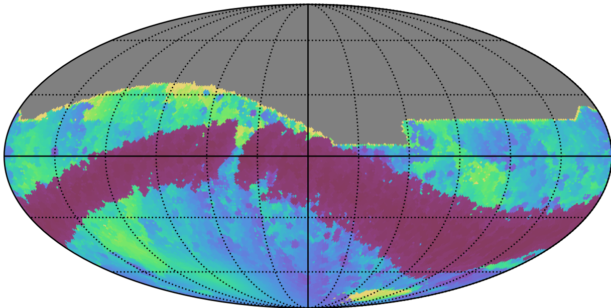
noroll_mjdp60_v3.4_10yrs All sky r band: Min solarElong
