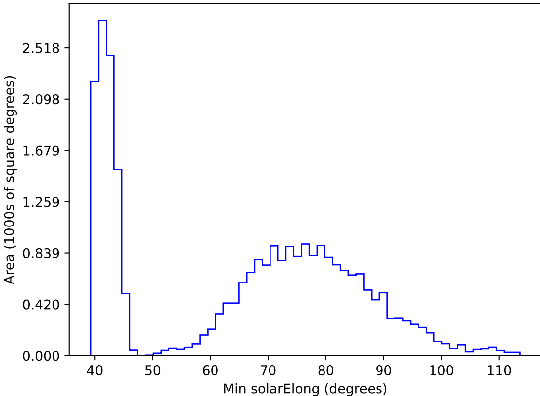
noroll_mjdp60_v3.4_10yrs All sky r band: Min solarElong
