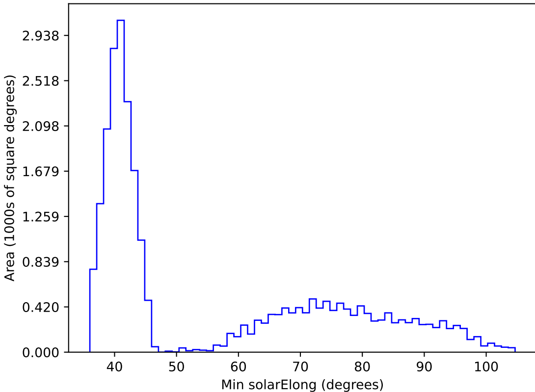
noroll_mjdp60_v3.4_10yrs All sky i band: Min solarElong
