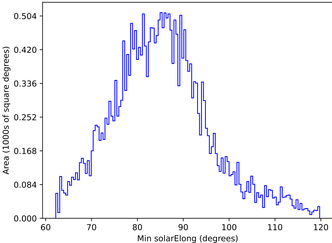
noroll_mjdp60_v3.4_10yrs All sky g band: Min solarElong
