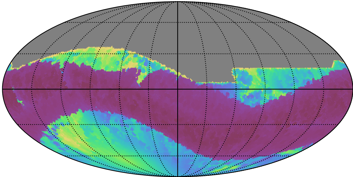
noroll_mjdp60_v3.4_10yrs All sky all bands: Min solarElong
