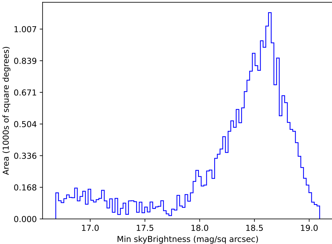
noroll_mjdp60_v3.4_10yrs Yr 1 z band: Min skyBrightness
