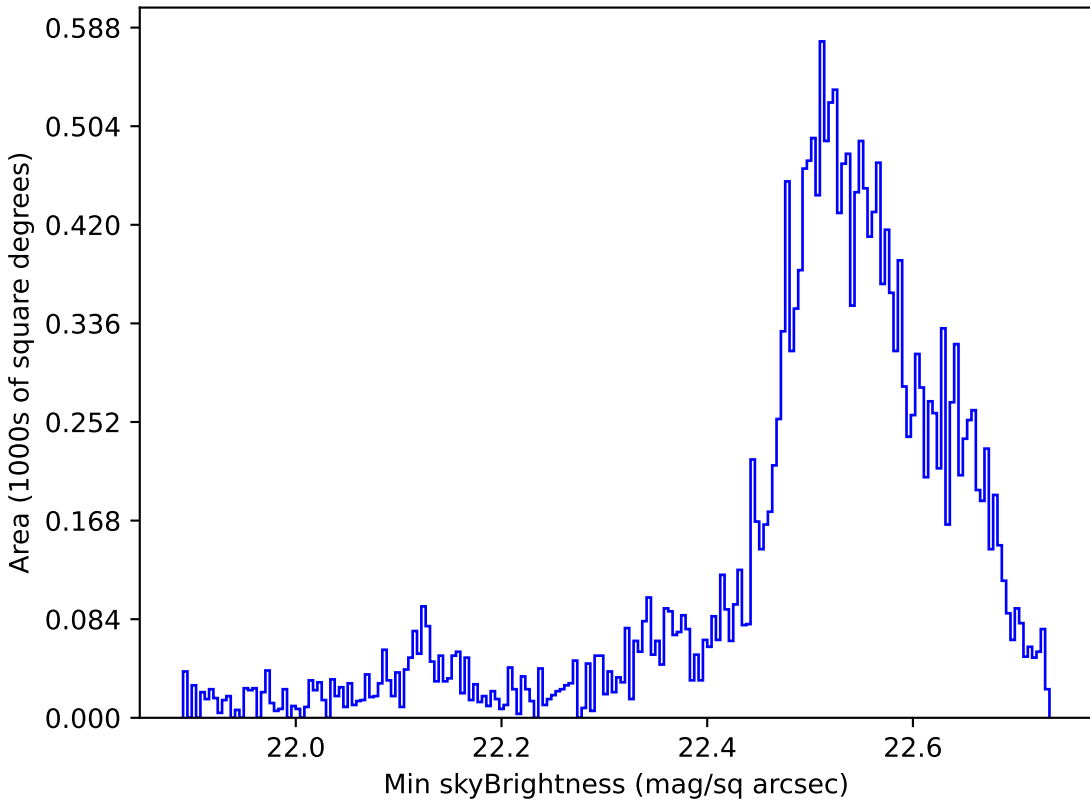
noroll_mjdp60_v3.4_10yrs Yr 1 u band: Min skyBrightness
