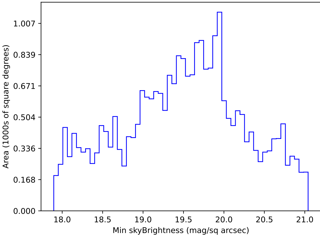
noroll_mjdp60_v3.4_10yrs Yr 1 r band: Min skyBrightness
