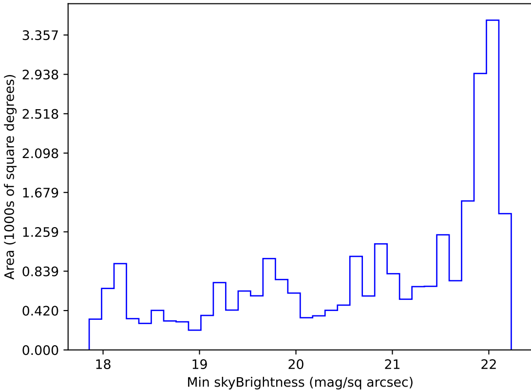
noroll_mjdp60_v3.4_10yrs Yr 1 g band: Min skyBrightness
