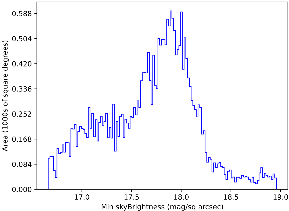
noroll_mjdp60_v3.4_10yrs Yr 1 all bands: Min skyBrightness
