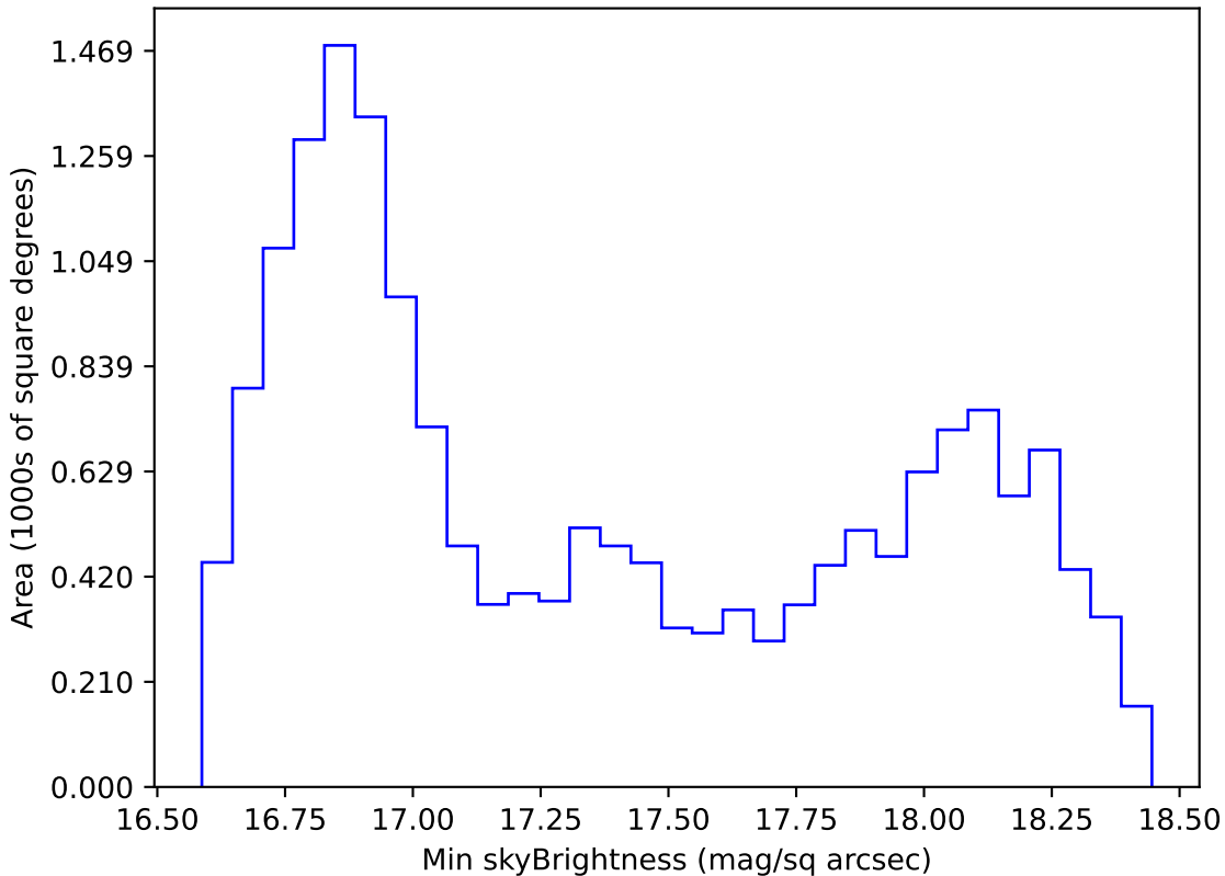
noroll_mjdp60_v3.4_10yrs WFD z band: Min skyBrightness
