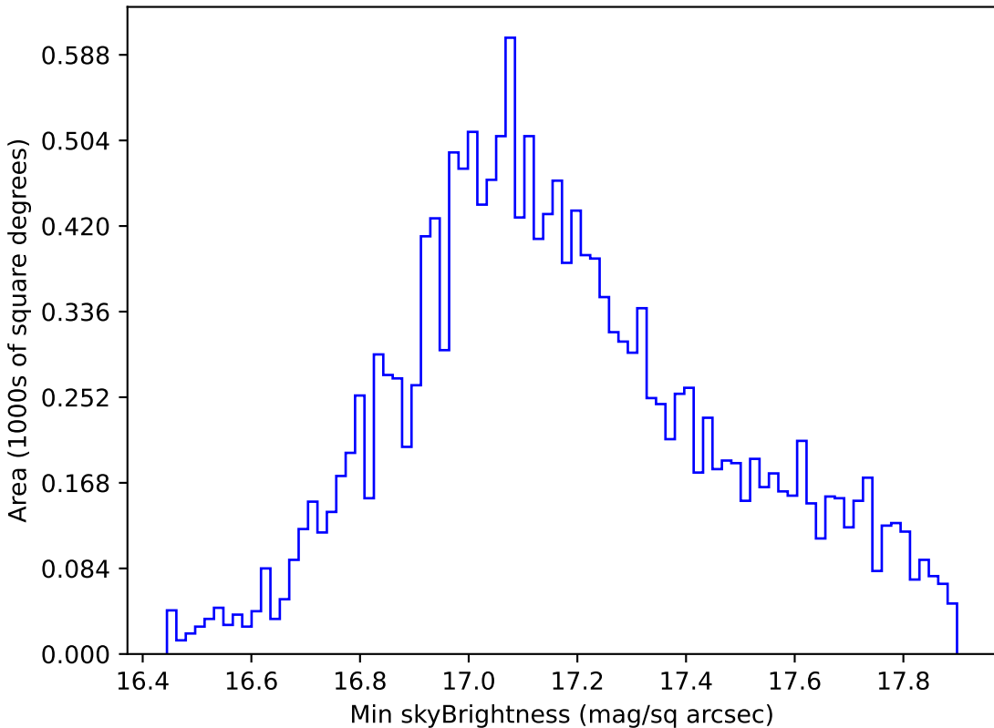
noroll_mjdp60_v3.4_10yrs WFD y band: Min skyBrightness
