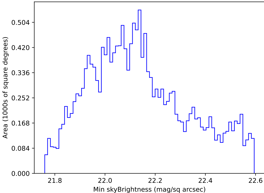
noroll_mjdp60_v3.4_10yrs WFD u band: Min skyBrightness
