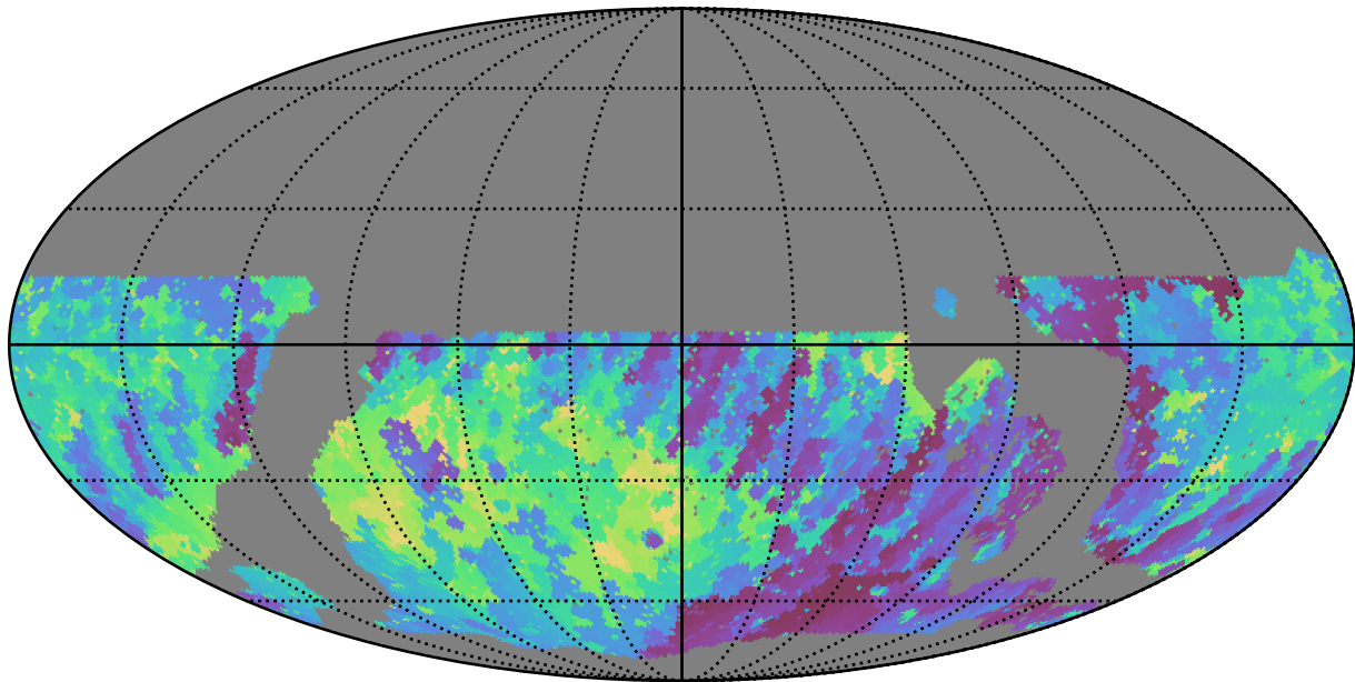
noroll_mjdp60_v3.4_10yrs WFD r band: Min skyBrightness
