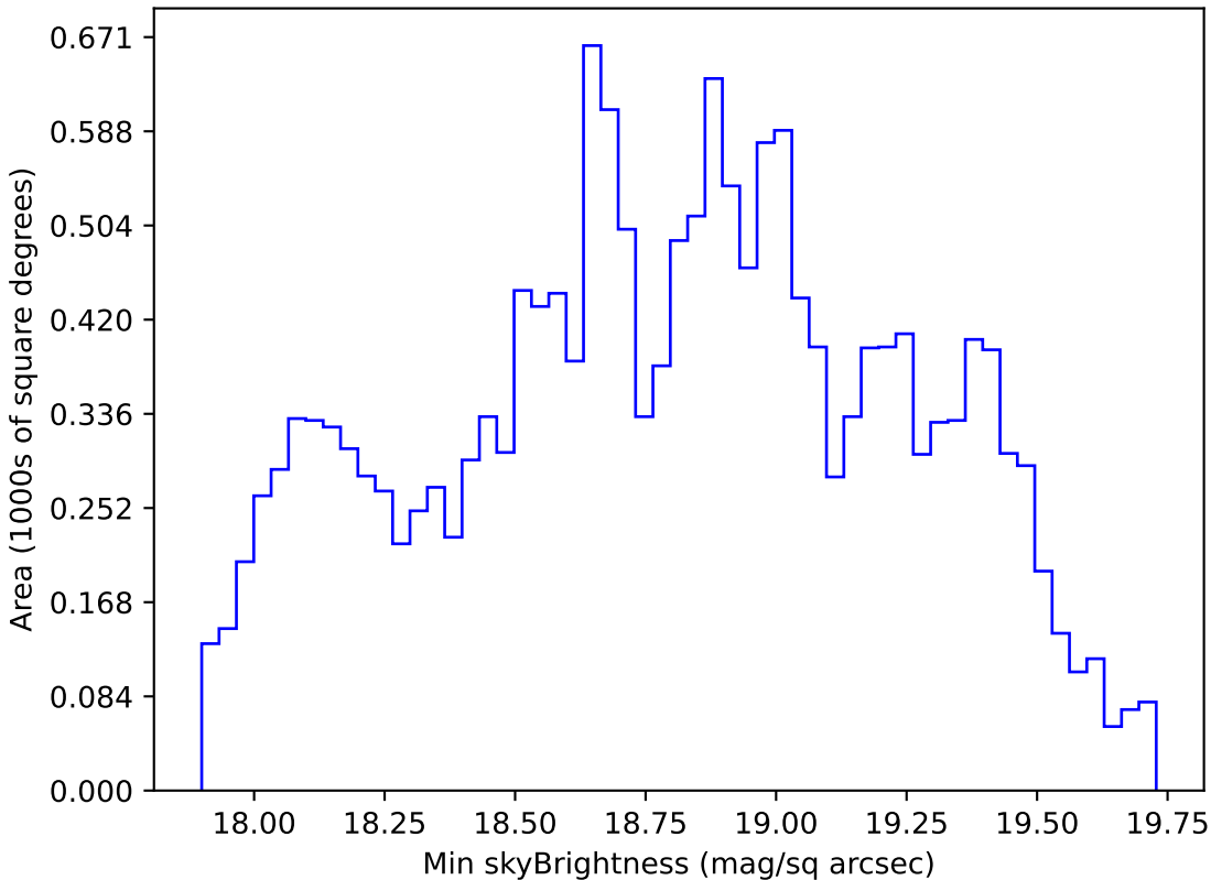
noroll_mjdp60_v3.4_10yrs WFD r band: Min skyBrightness
