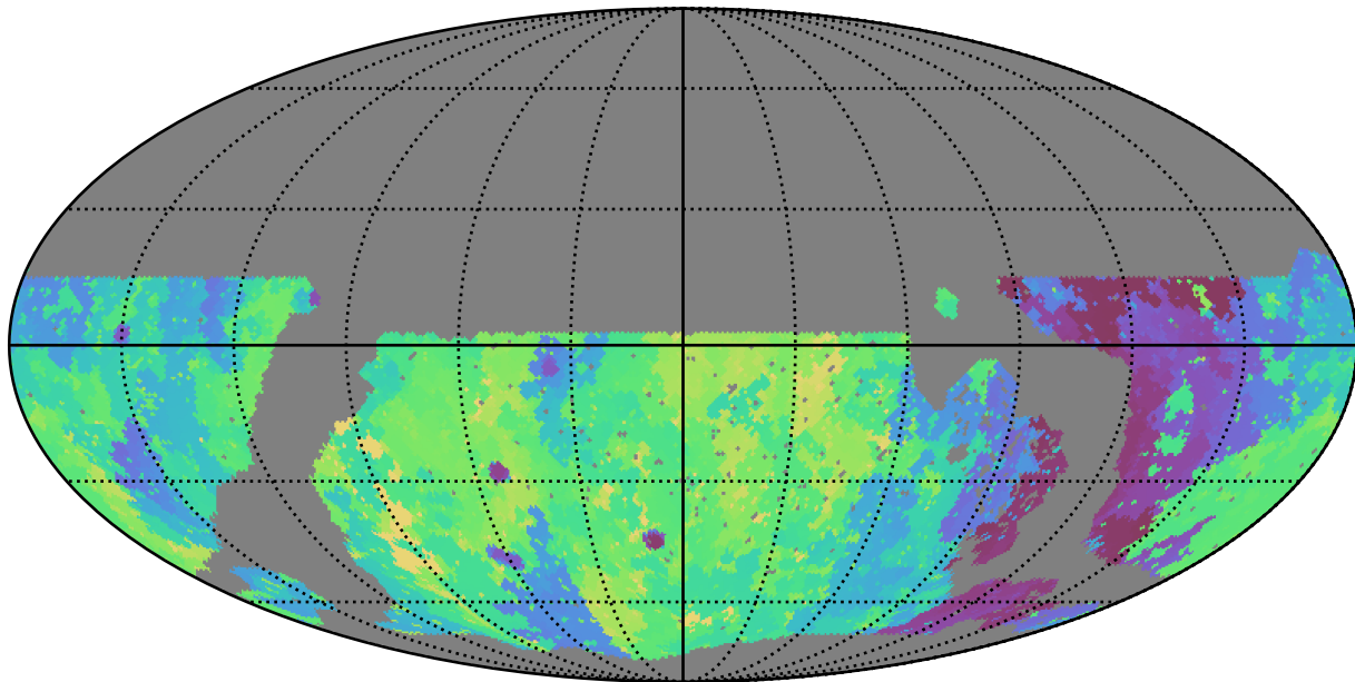
noroll_mjdp60_v3.4_10yrs WFD g band: Min skyBrightness
