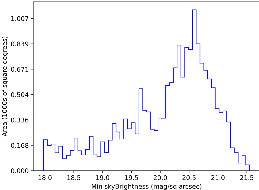
noroll_mjdp60_v3.4_10yrs WFD g band: Min skyBrightness
