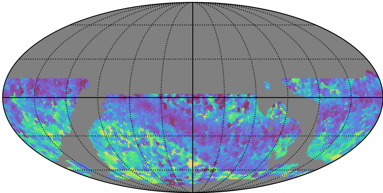
noroll_mjdp60_v3.4_10yrs WFD all bands: Min skyBrightness
