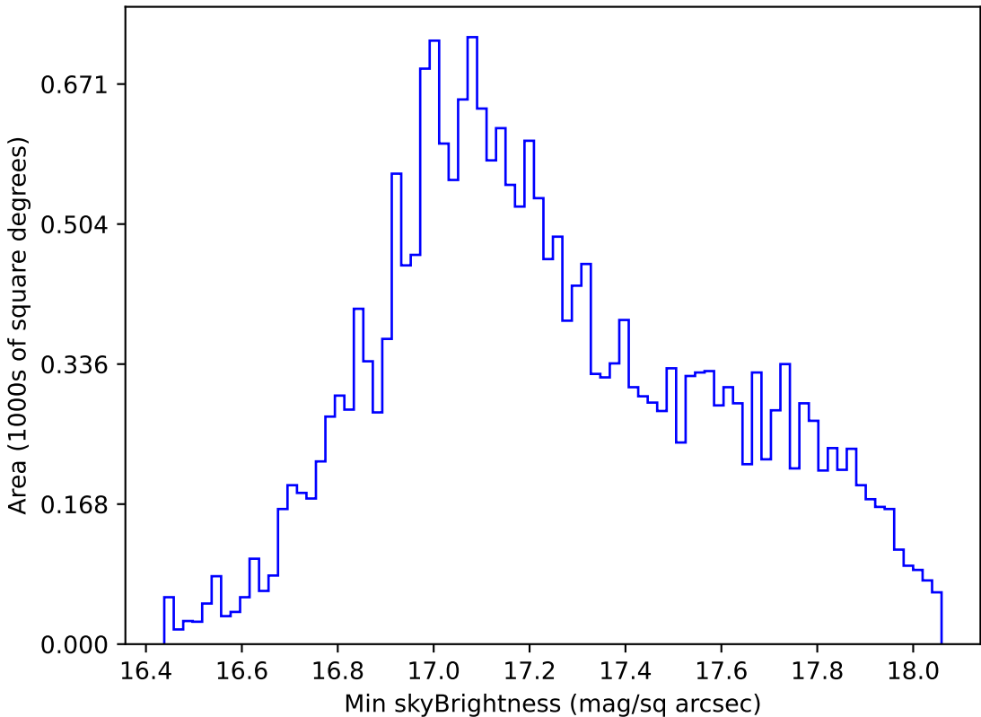
noroll_mjdp60_v3.4_10yrs All sky y band: Min skyBrightness
