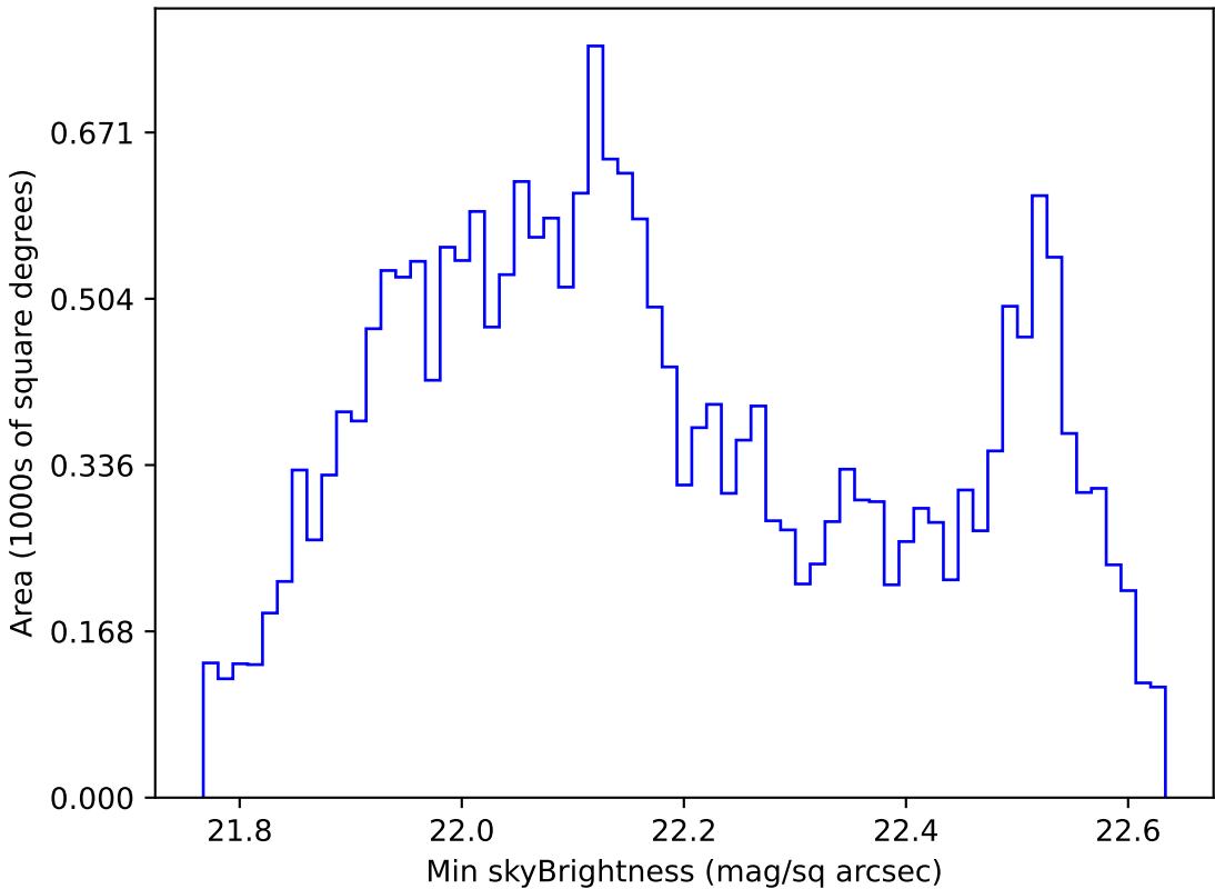
noroll_mjdp60_v3.4_10yrs All sky u band: Min skyBrightness
