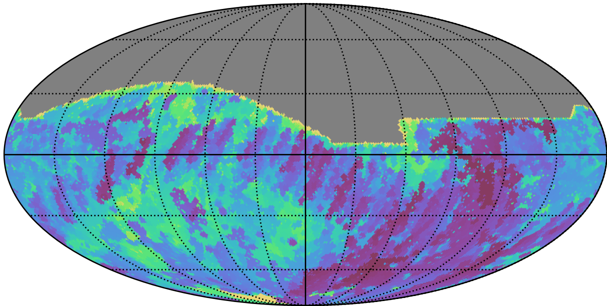
noroll_mjdp60_v3.4_10yrs All sky r band: Min skyBrightness
