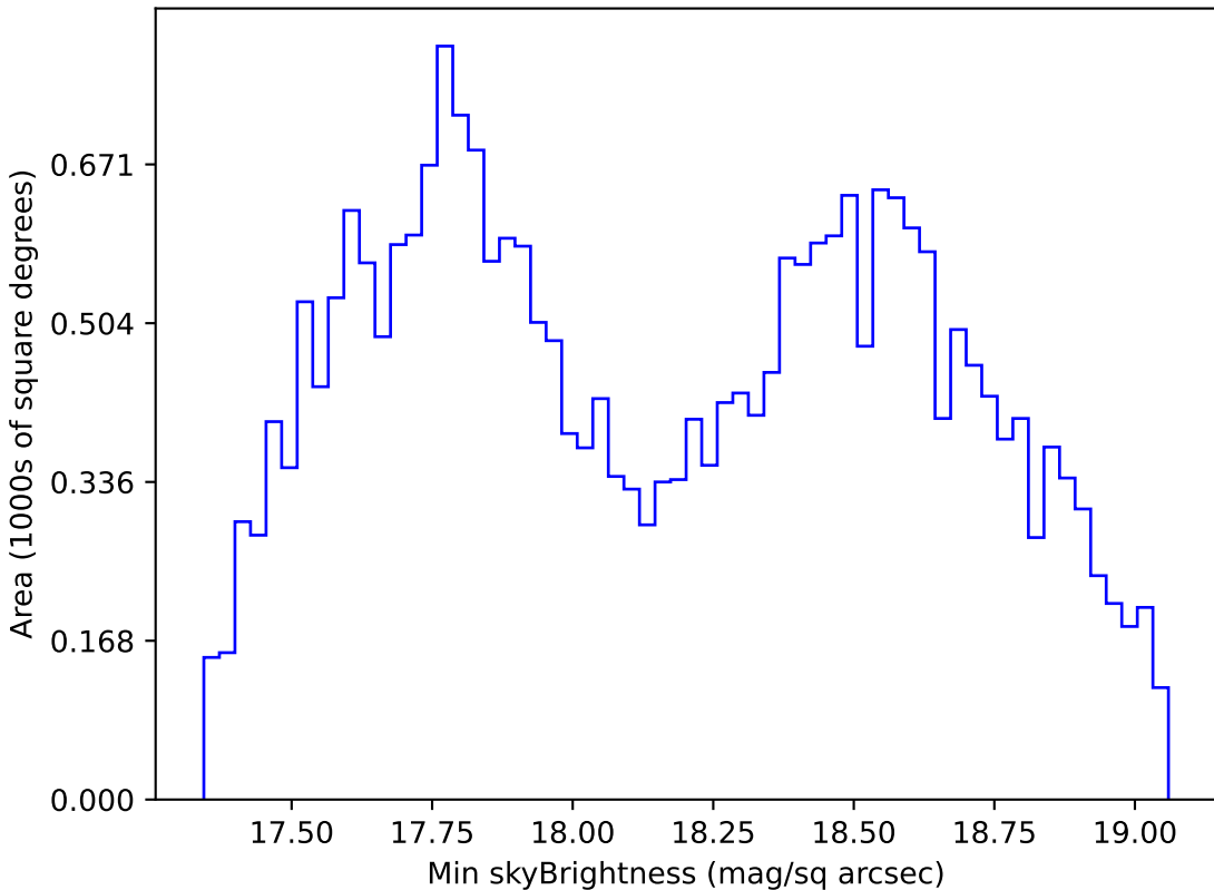
noroll_mjdp60_v3.4_10yrs All sky i band: Min skyBrightness
