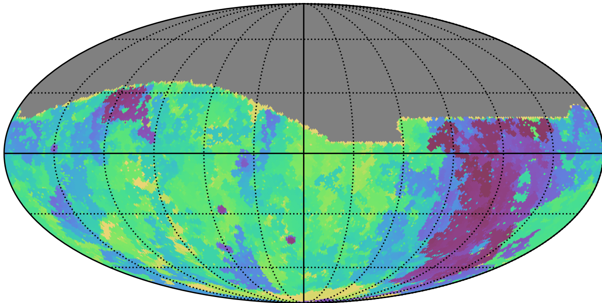
noroll_mjdp60_v3.4_10yrs All sky g band: Min skyBrightness
