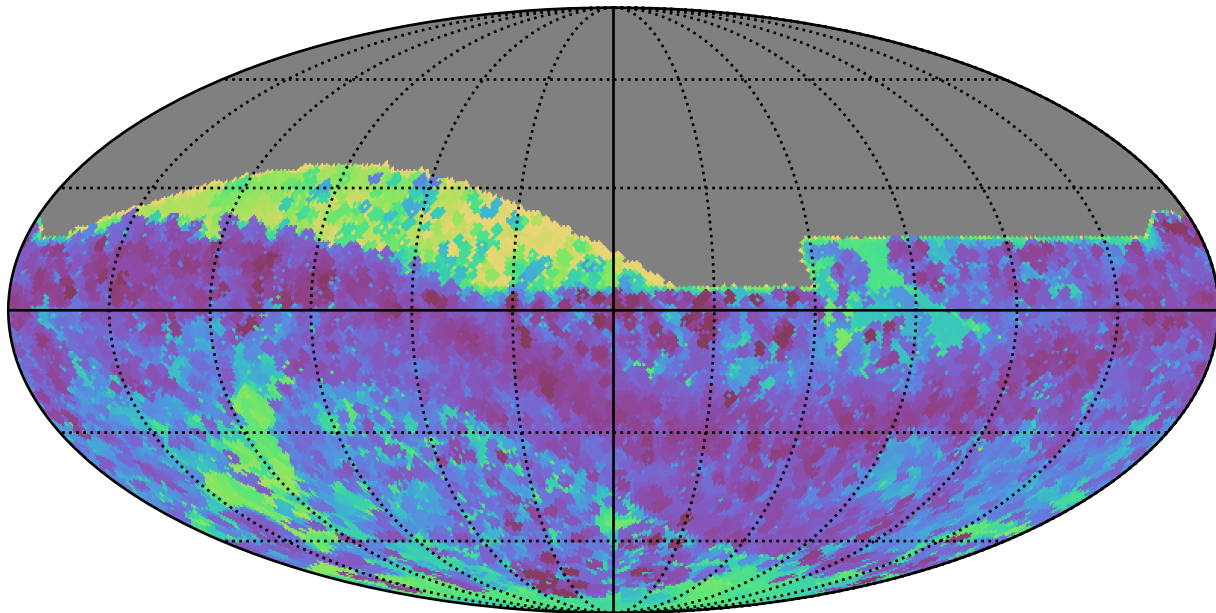
noroll_mjdp60_v3.4_10yrs All sky all bands: Min skyBrightness
