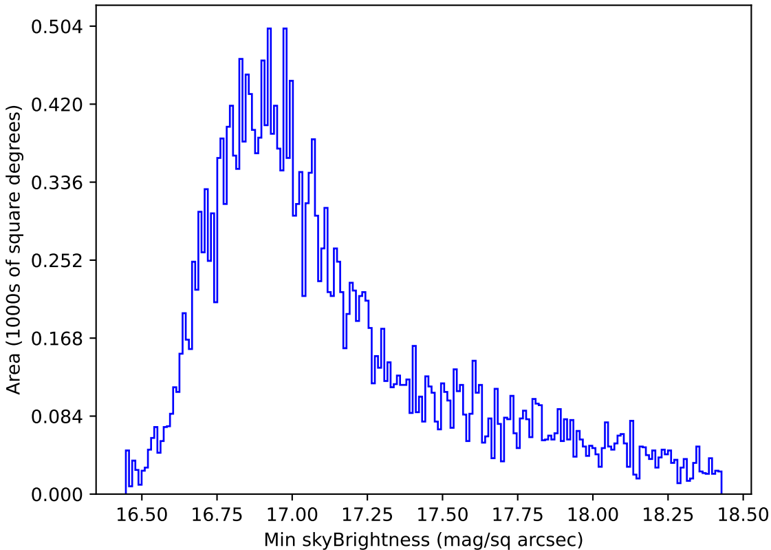
noroll_mjdp60_v3.4_10yrs All sky all bands: Min skyBrightness
