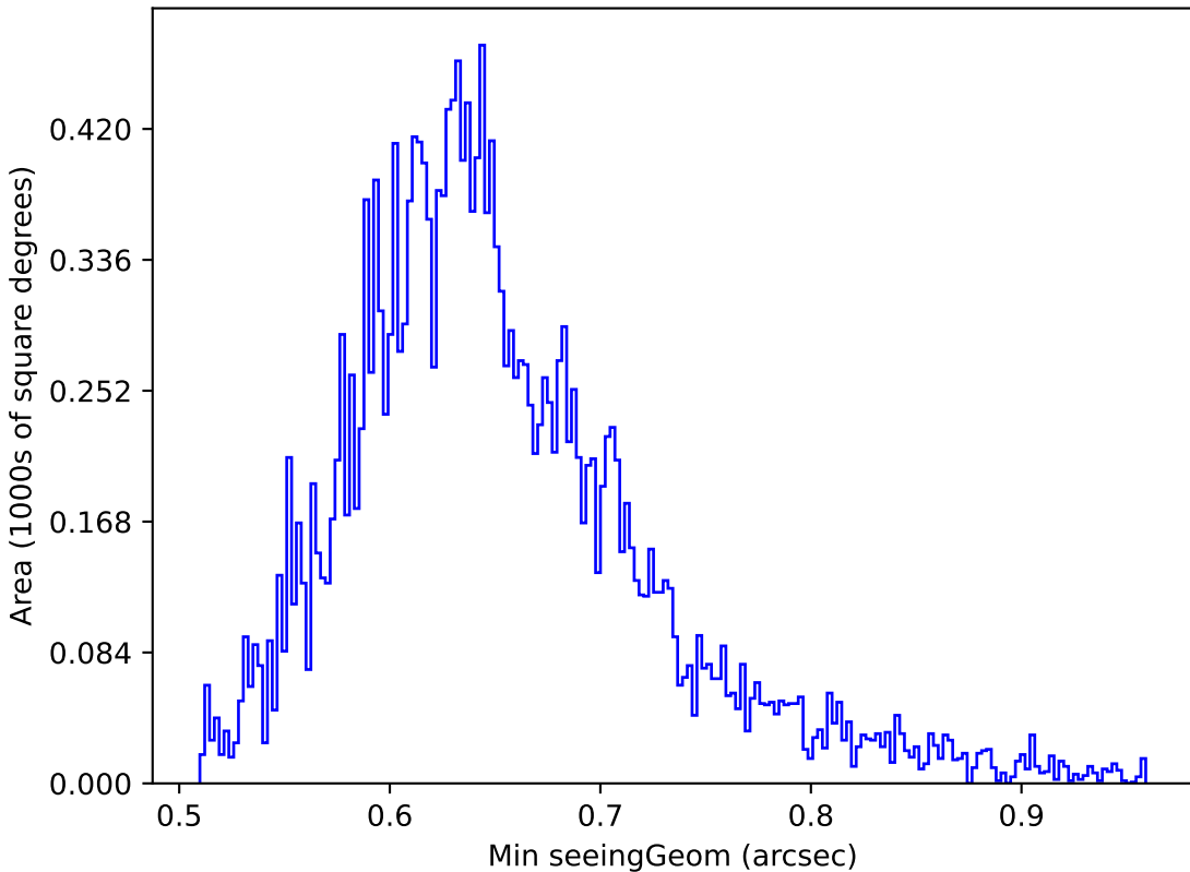
noroll_mjdp60_v3.4_10yrs Yr 1 y band: Min seeingGeom
