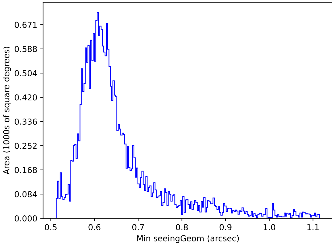
noroll_mjdp60_v3.4_10yrs Yr 1 r band: Min seeingGeom
