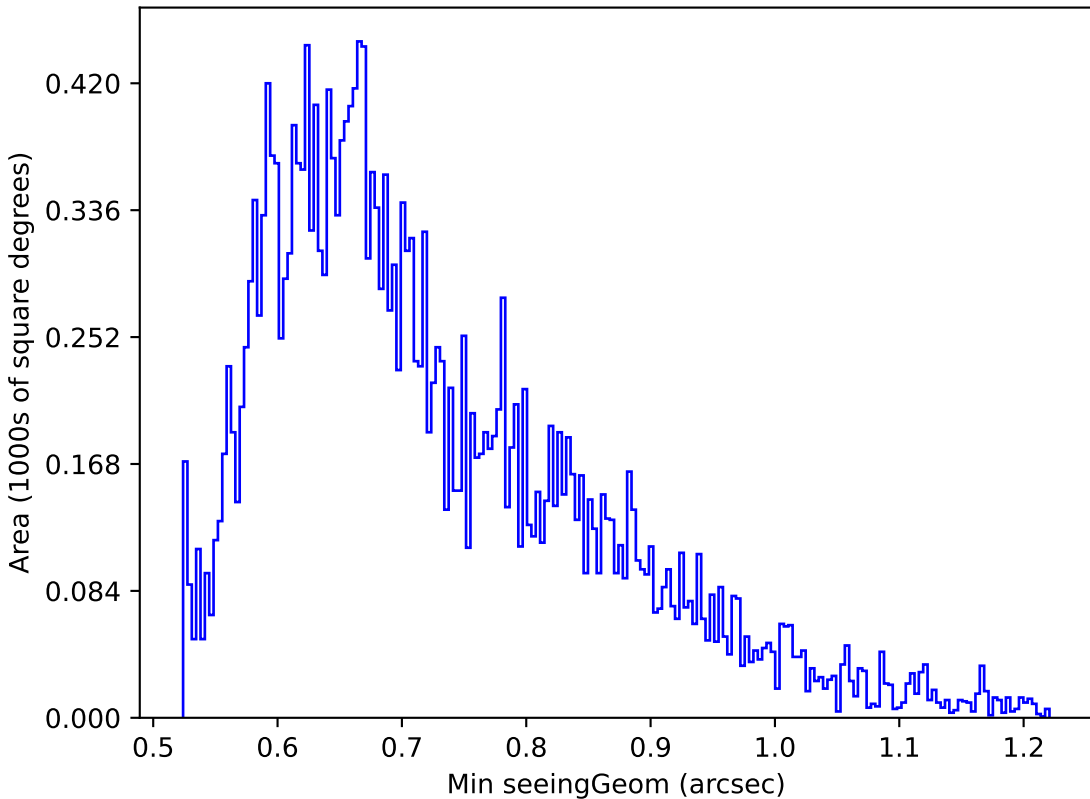
noroll_mjdp60_v3.4_10yrs Yr 1 g band: Min seeingGeom
