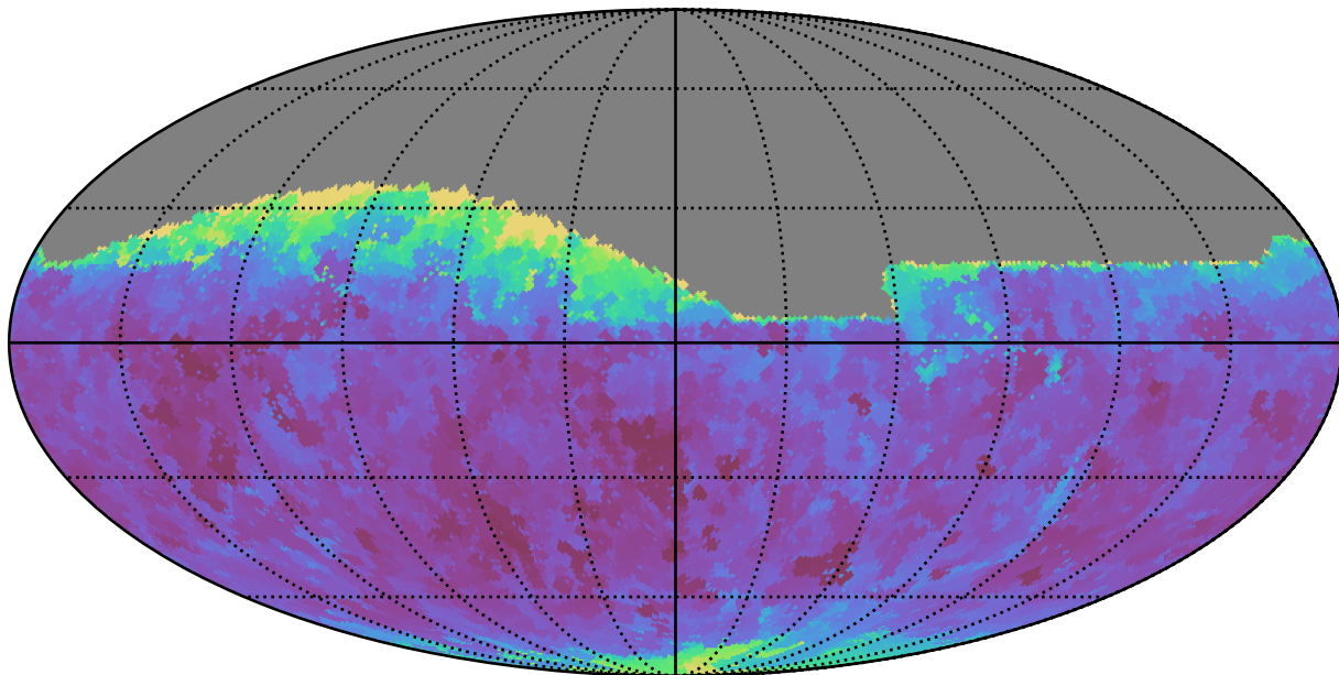
noroll_mjdp60_v3.4_10yrs Yr 1 all bands: Min seeingGeom
