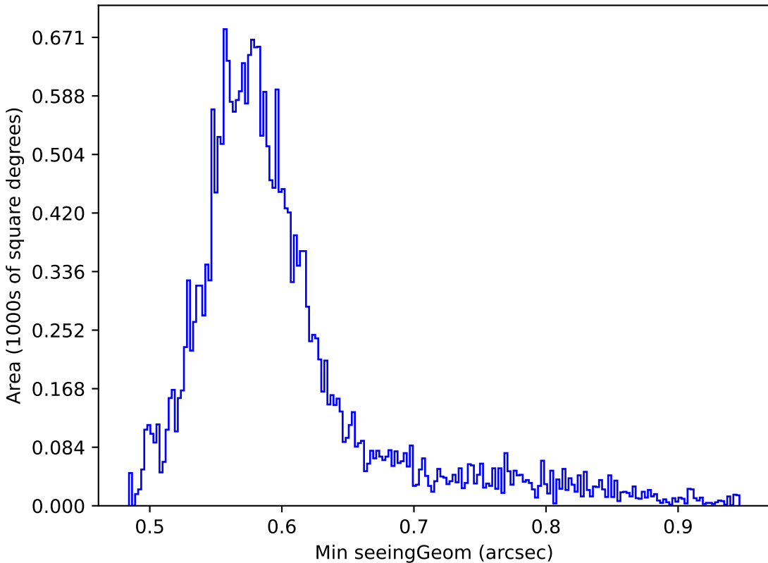
noroll_mjdp60_v3.4_10yrs Yr 1 all bands: Min seeingGeom
